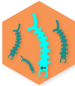
LARVA
